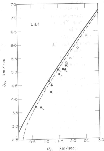
Fig. 3. Hugoniot of LiBr. — lattice model calculation. --- model calculation for 2 per cent porous sample. ○ Single Crystal Experiment[60]; ● Pressed Sample[61], corrected to single crystal Hugoniot.
